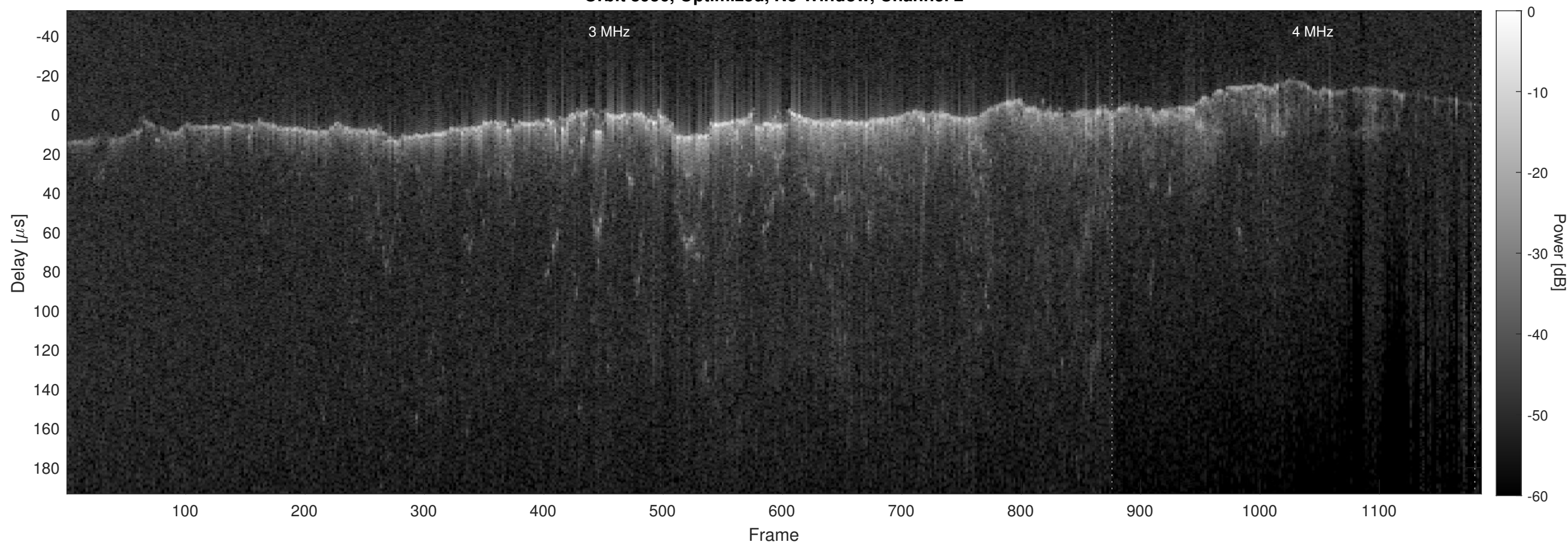
Orbit 8956, Optimized, No Window, Channel 2
