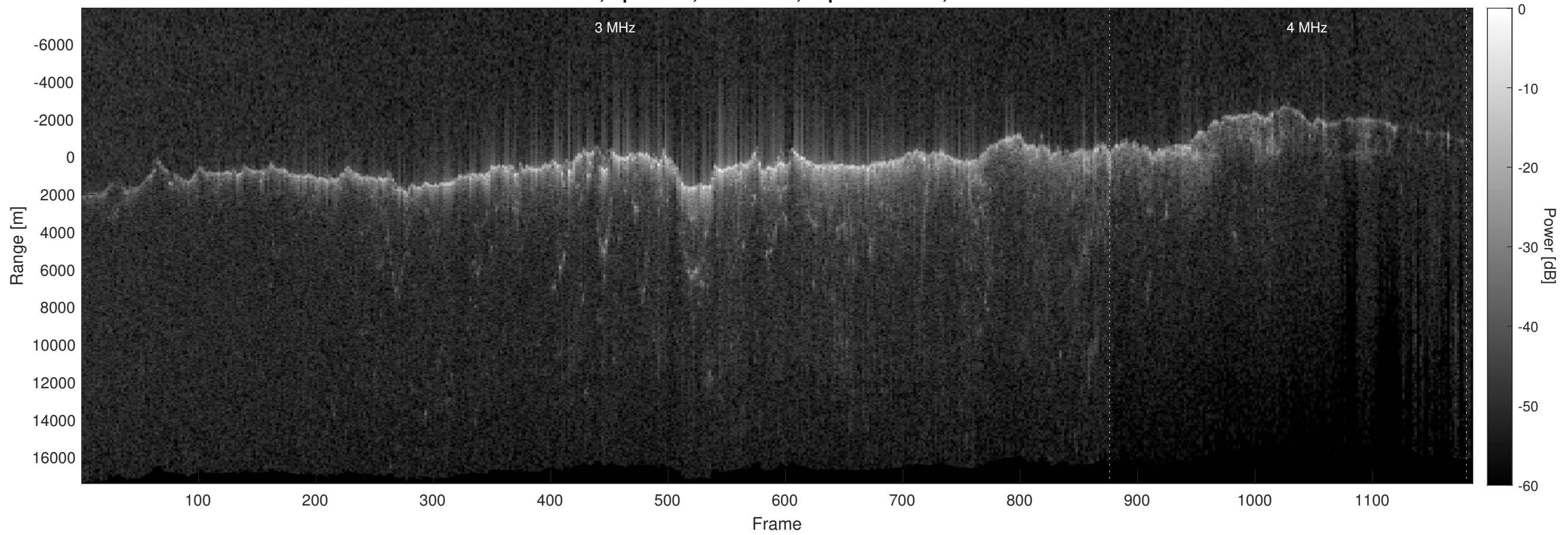
Orbit 8956, Optimized, No Window, Depth-Corrected, Channel 2
