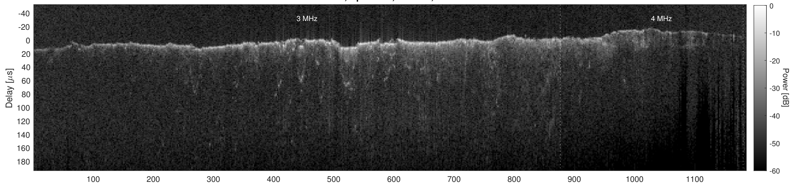
Orbit 8956, Cluttergram
