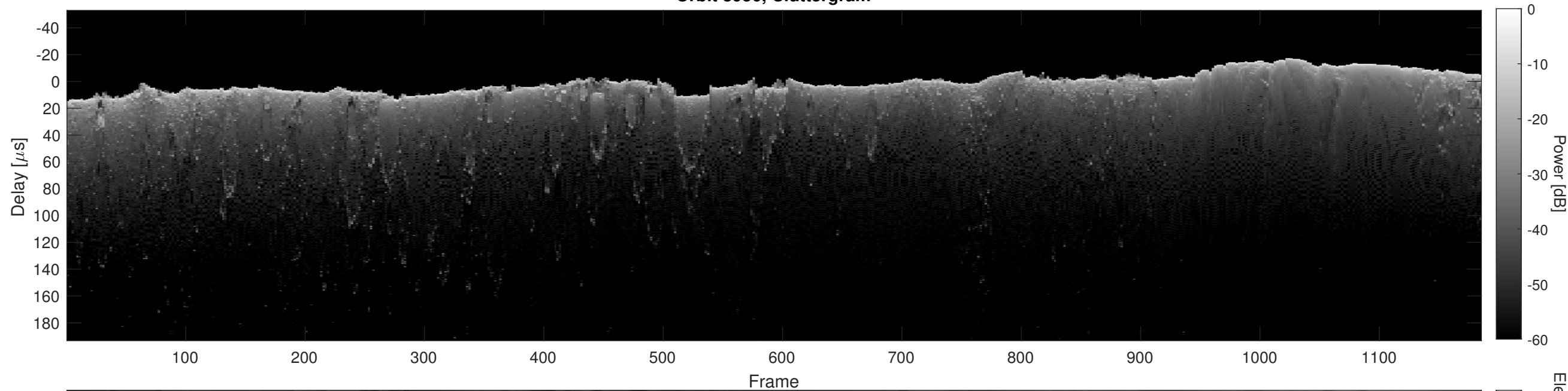
Orbit 8956, Cluttergram
