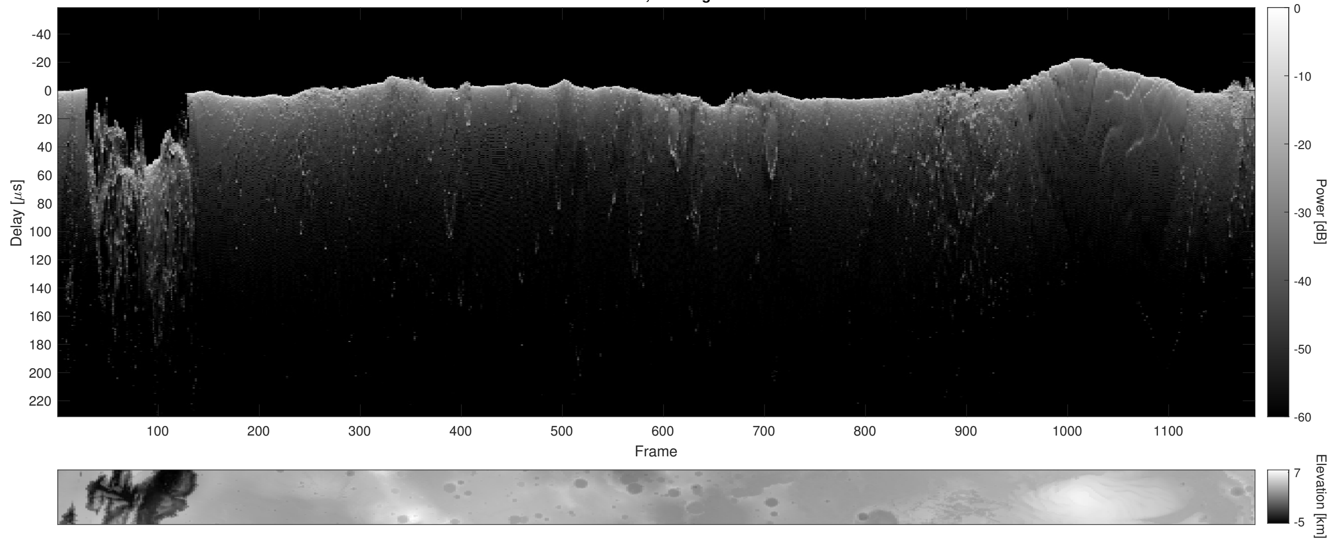
Orbit 8957, Cluttergram
