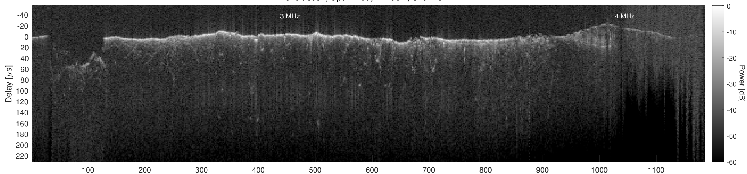
Orbit 8957, Cluttergram
