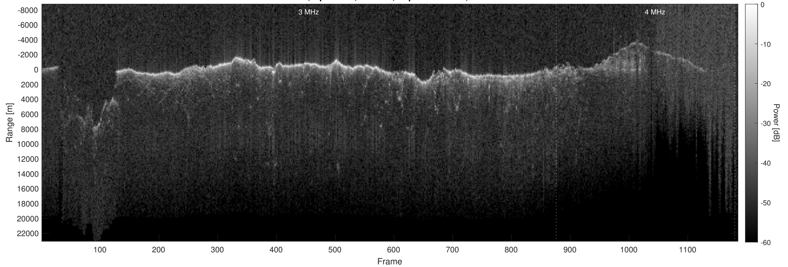
Orbit 8957, Optimized, Window, Depth-Corrected, Channel 2
