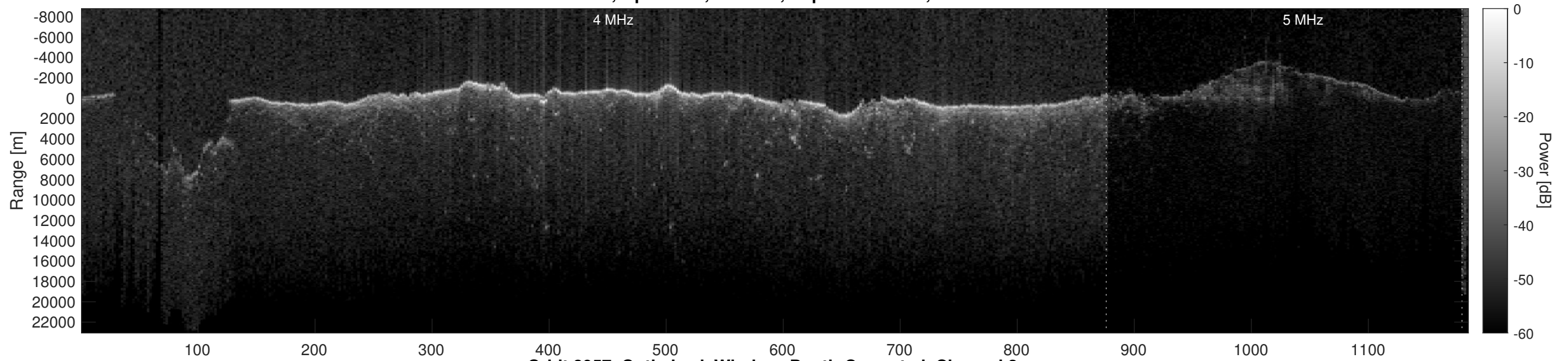
Orbit 8957, Optimized, Window, Depth-Corrected, Channel 2
