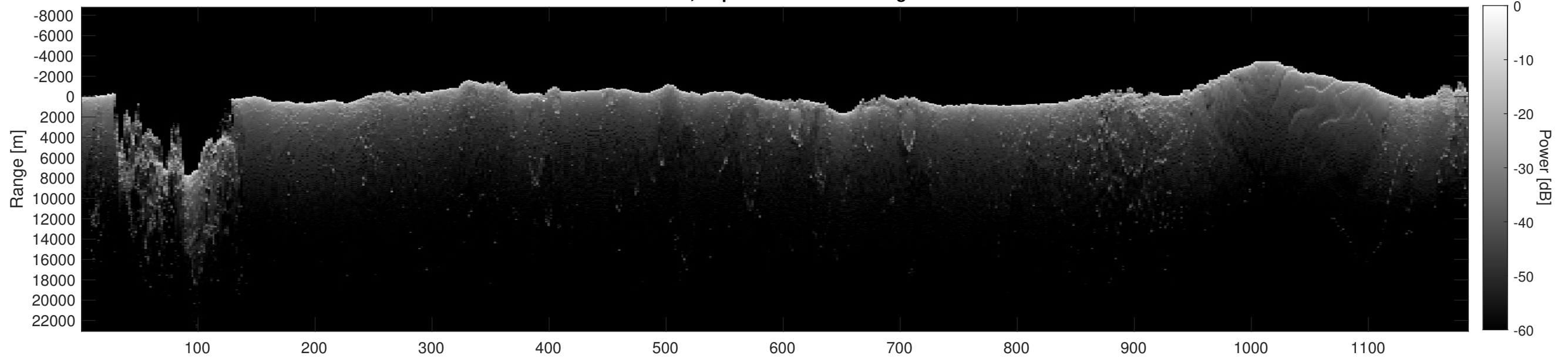
Orbit 8957, Depth-Corrected Cluttergram
