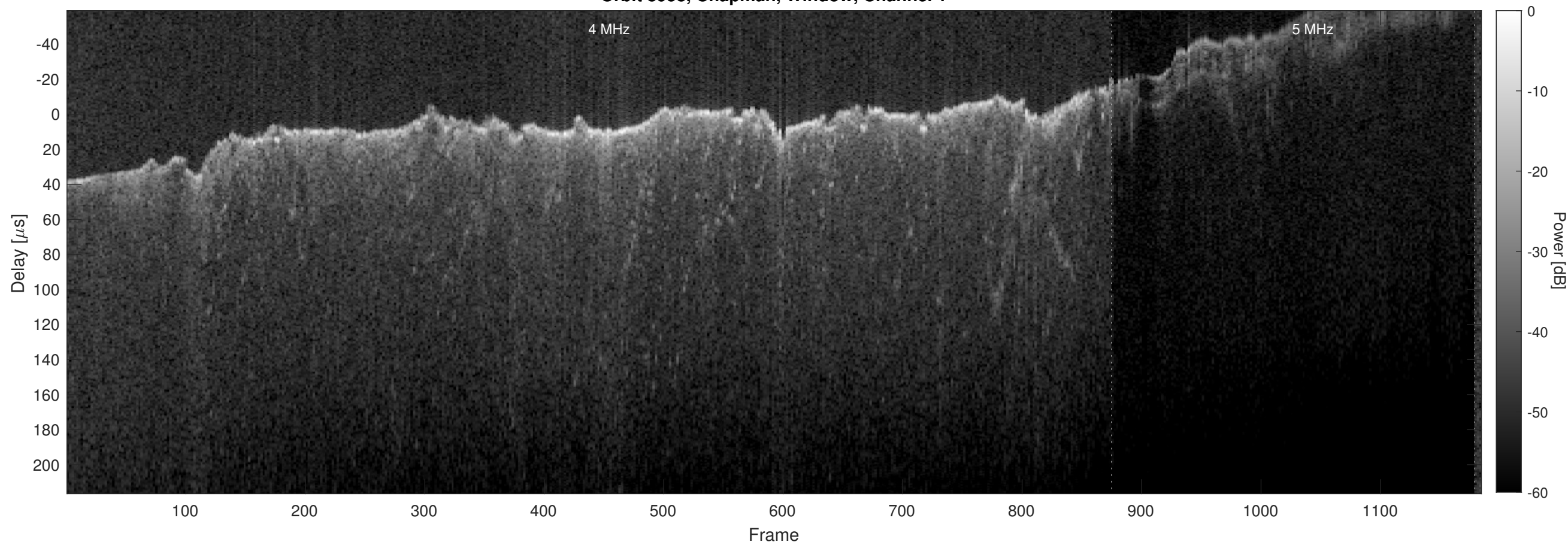
Orbit 8958, Chapman, Window, Channel 2
