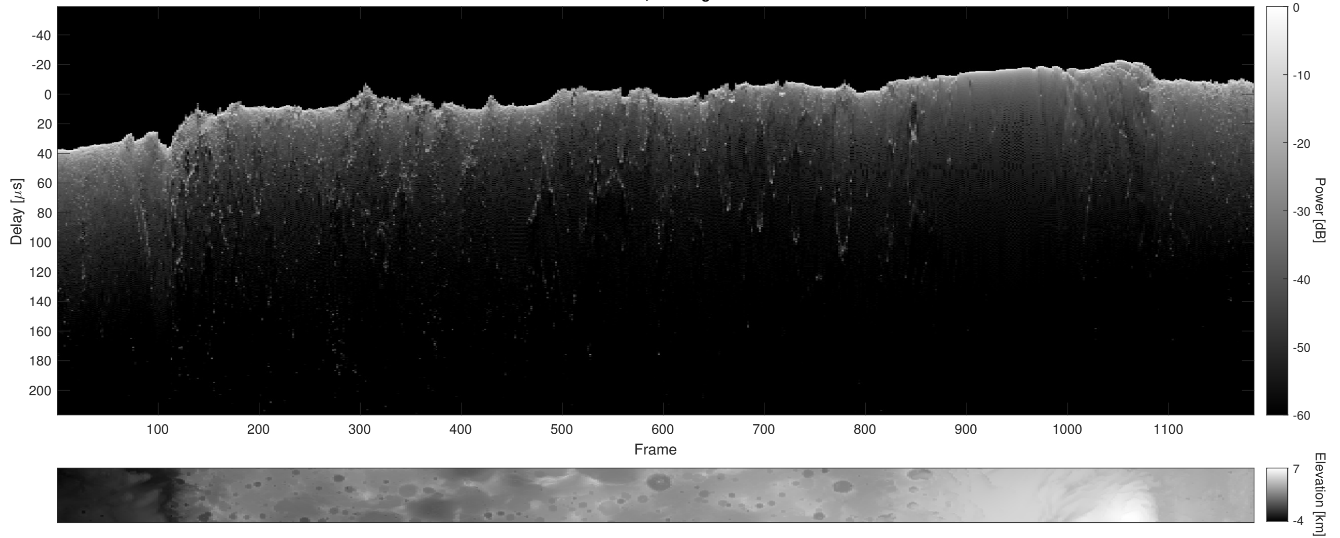
Orbit 8958, Cluttergram
