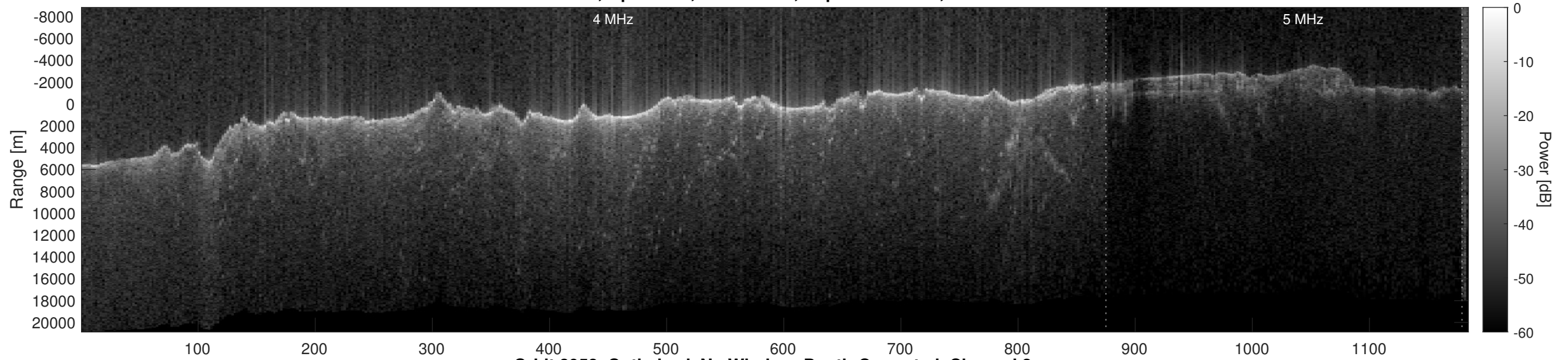
Orbit 8958, Optimized, No Window, Depth-Corrected, Channel 2
