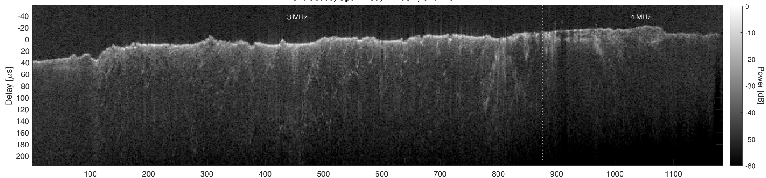
Orbit 8958, Cluttergram
