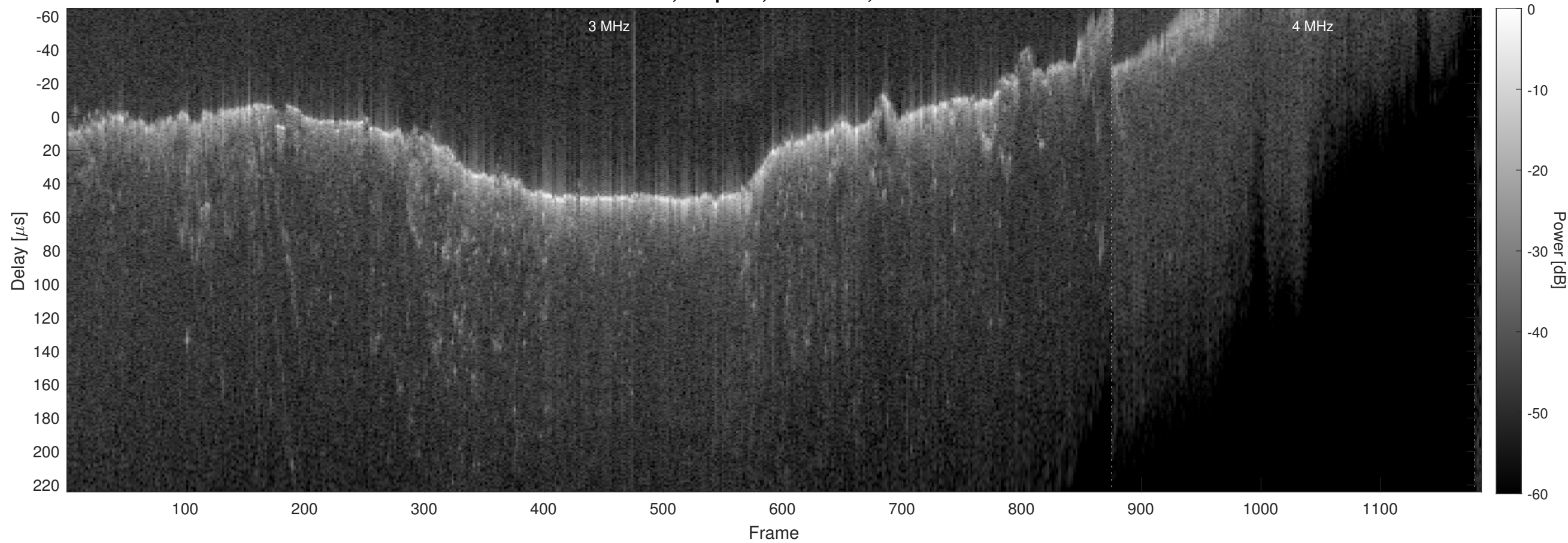
Orbit 8959, Chapman, No Window, Channel 2
