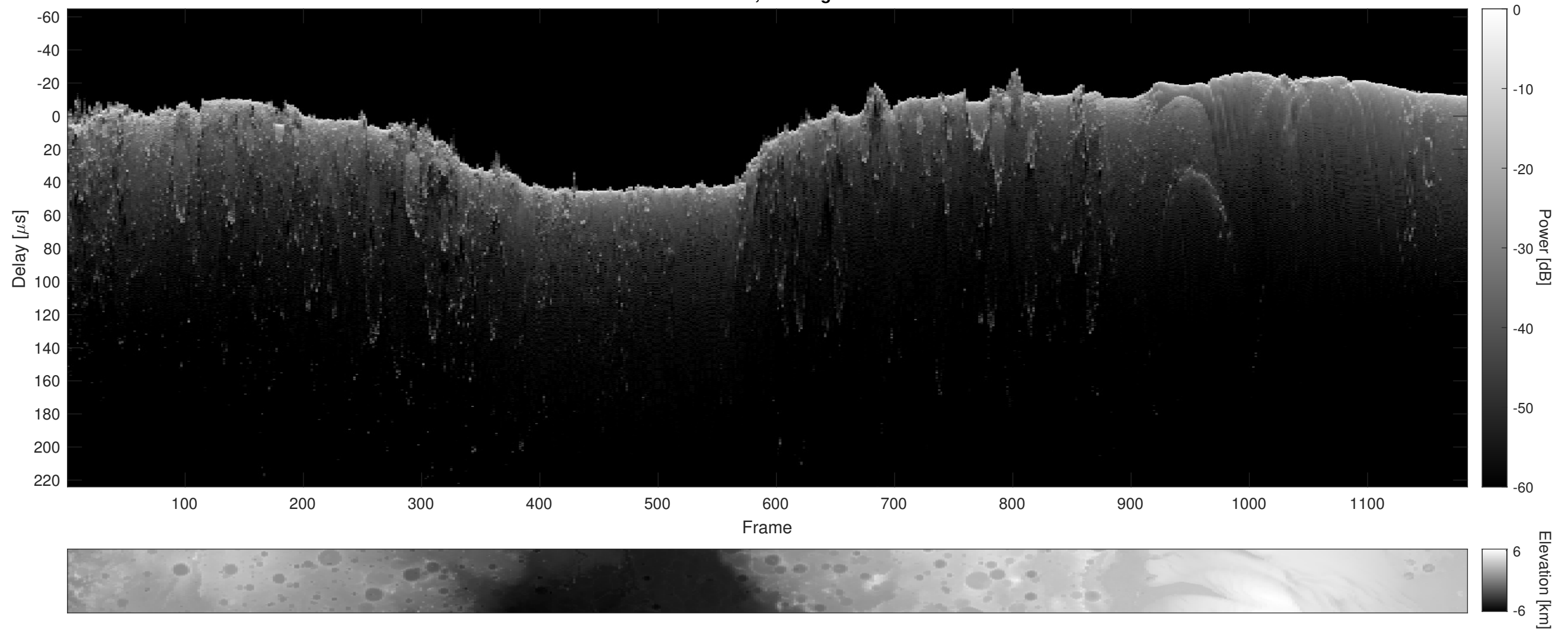
Orbit 8959, Cluttergram
