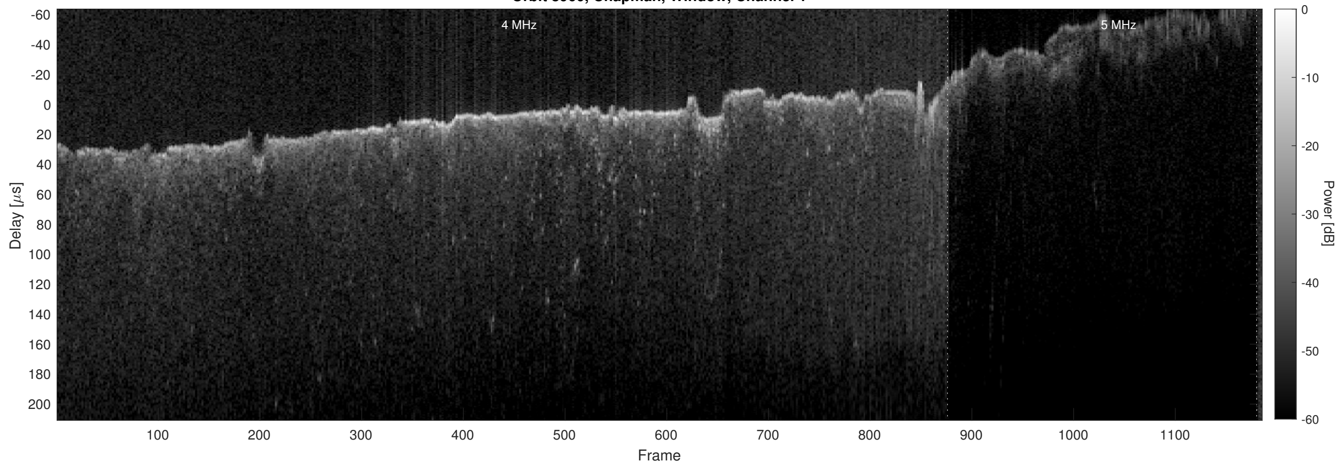
Orbit 8960, Chapman, Window, Channel 2
