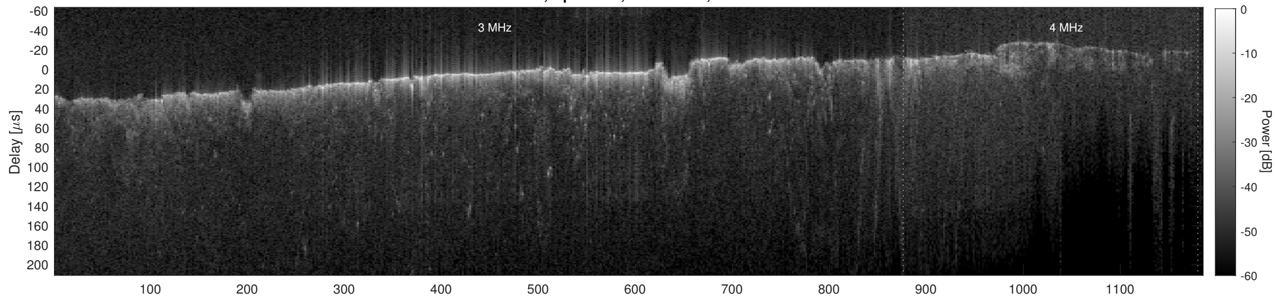
Orbit 8960, Cluttergram
