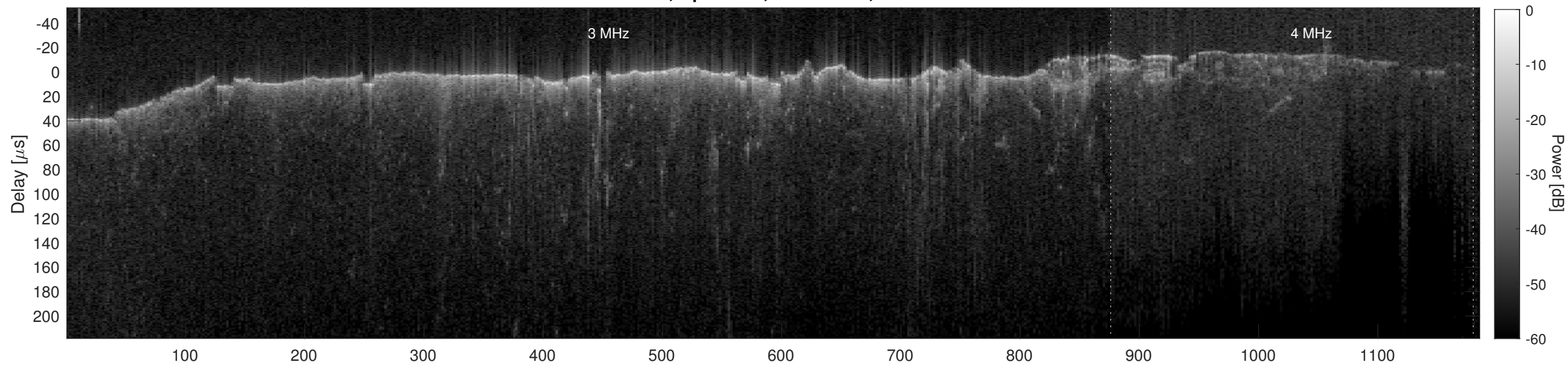
Orbit 8962, Cluttergram
