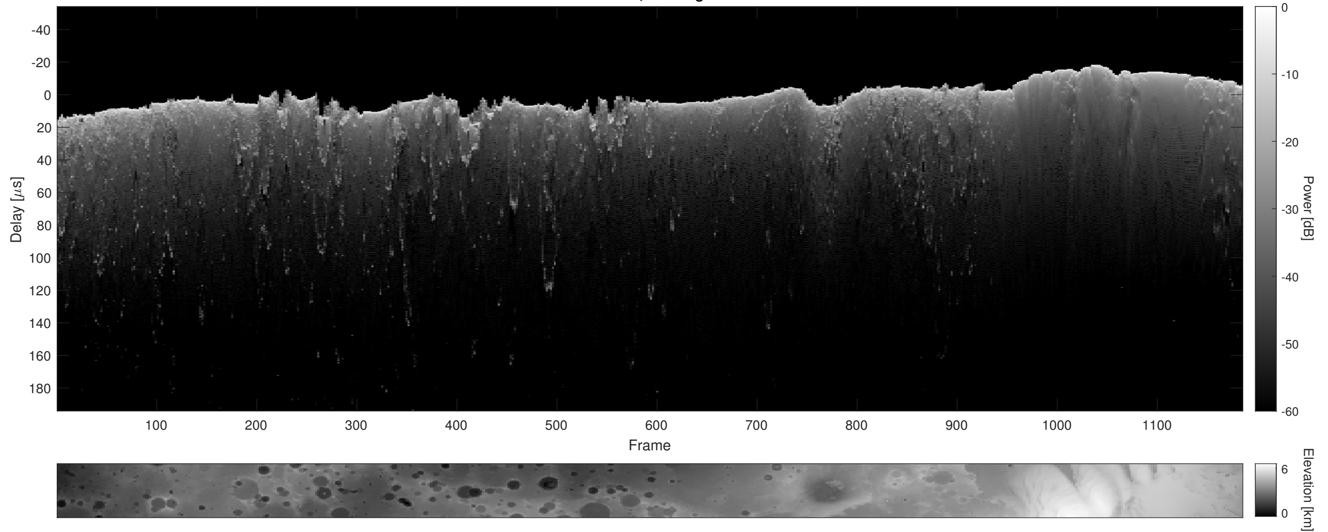
Orbit 8963, Cluttergram
