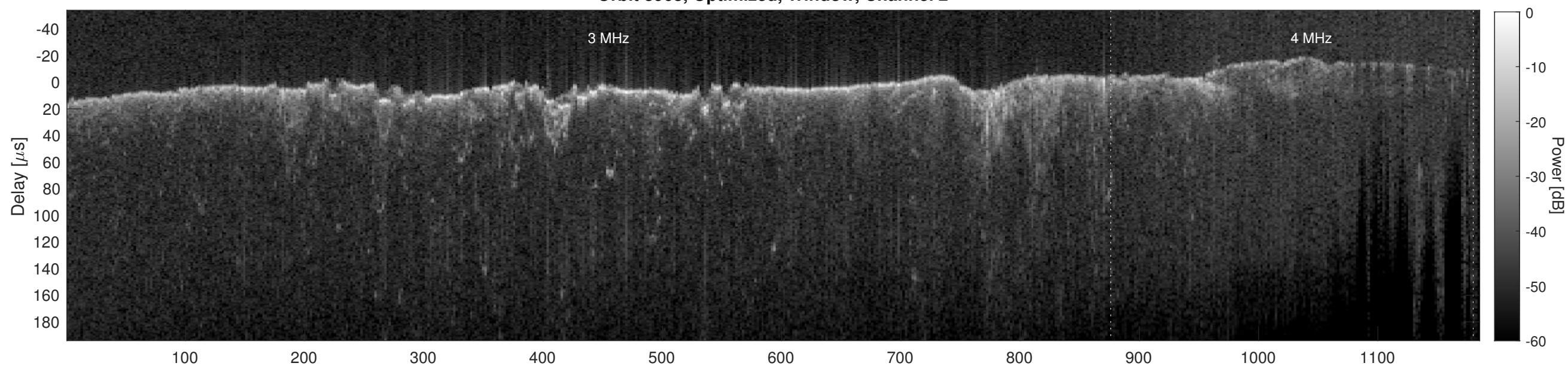
Orbit 8963, Cluttergram
