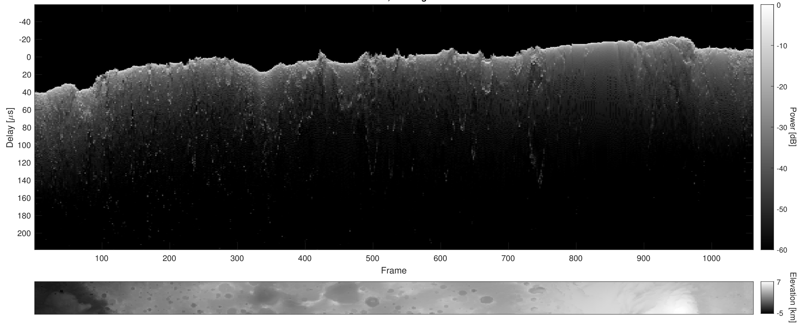
Orbit 8965, Cluttergram
