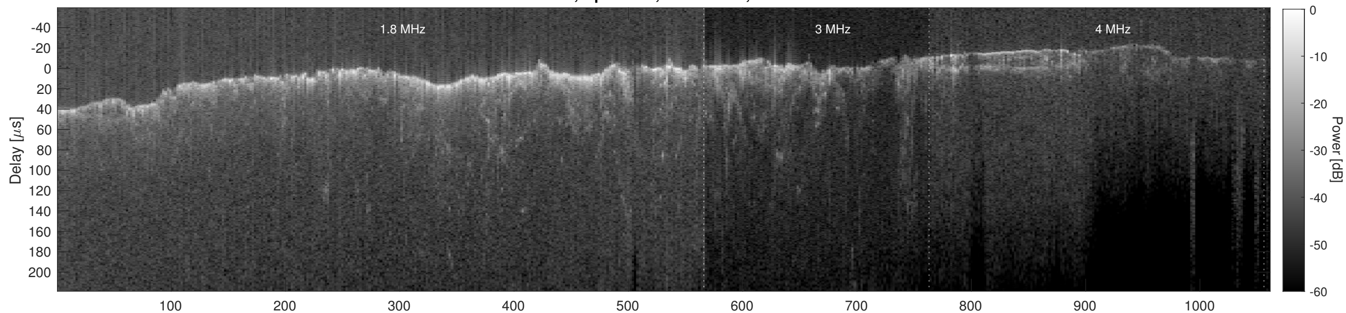
Orbit 8965, Cluttergram
