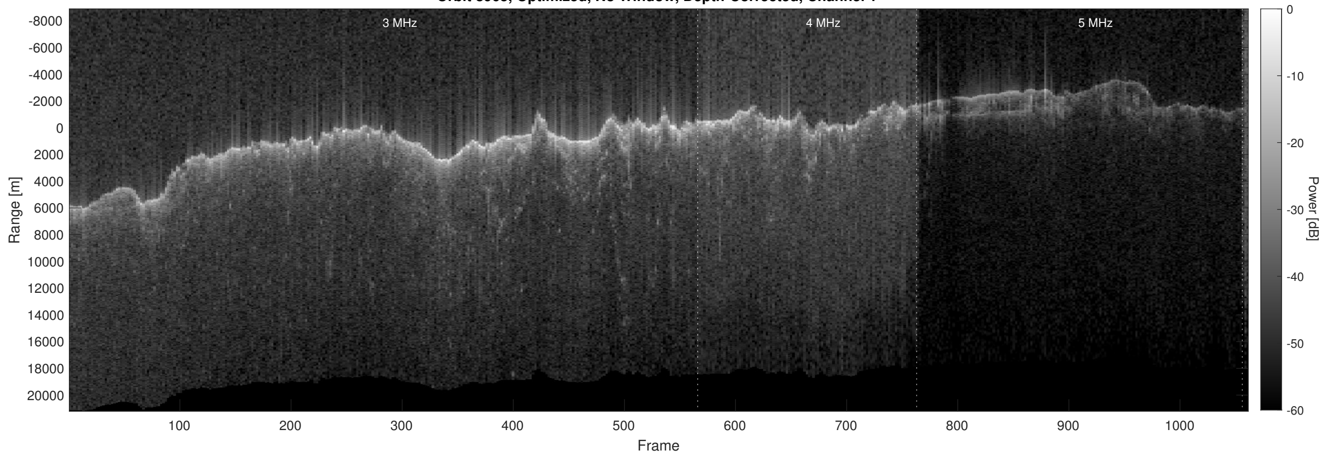
Orbit 8965, Optimized, No Window, Depth-Corrected, Channel 2
