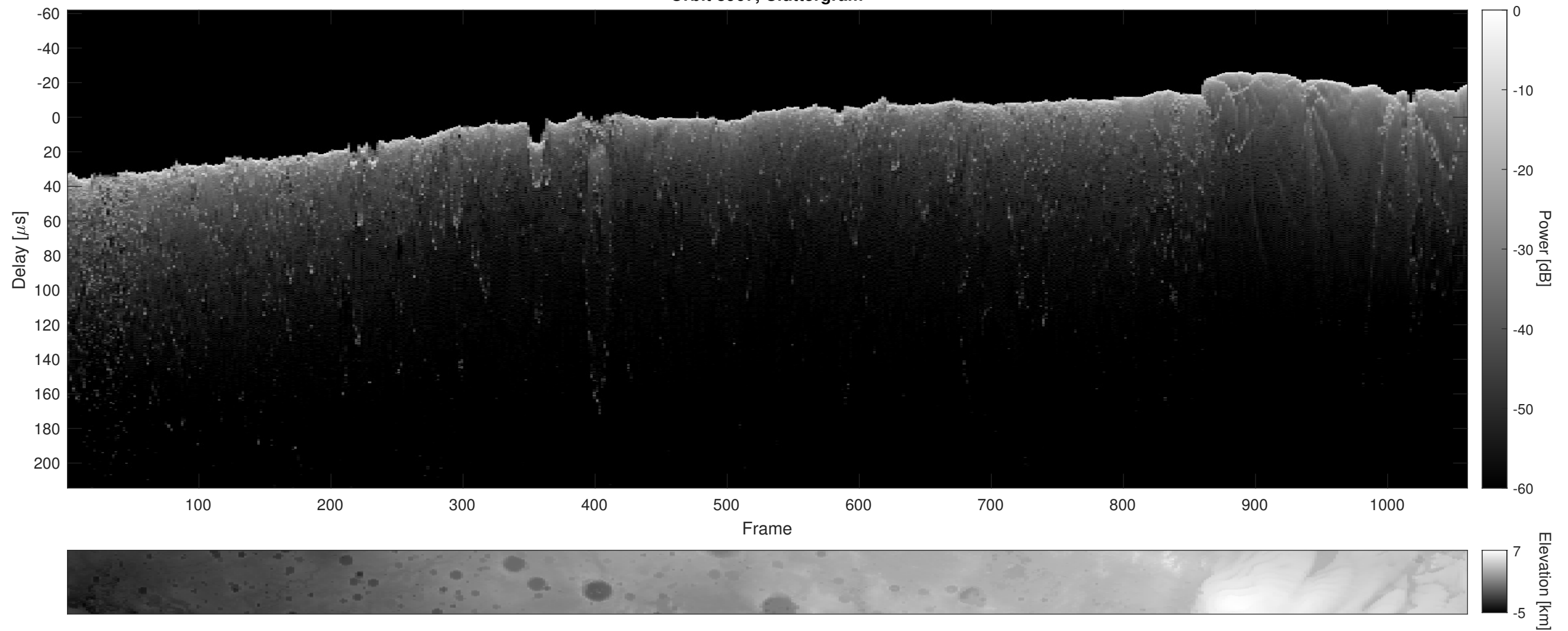
Orbit 8967, Cluttergram
