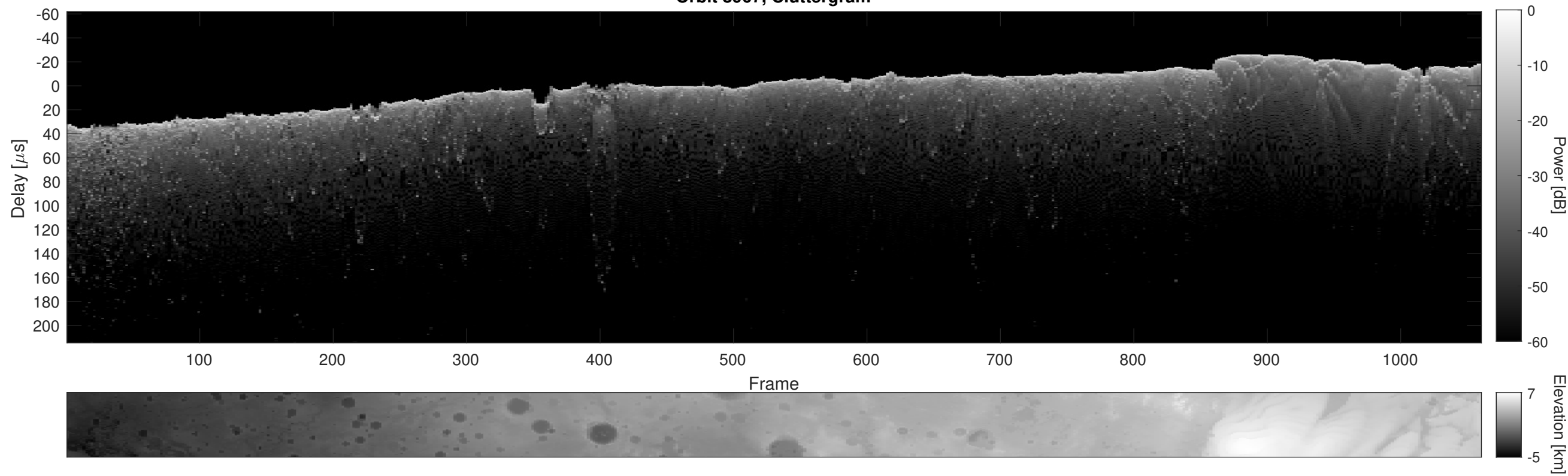
Orbit 8967, Cluttergram
