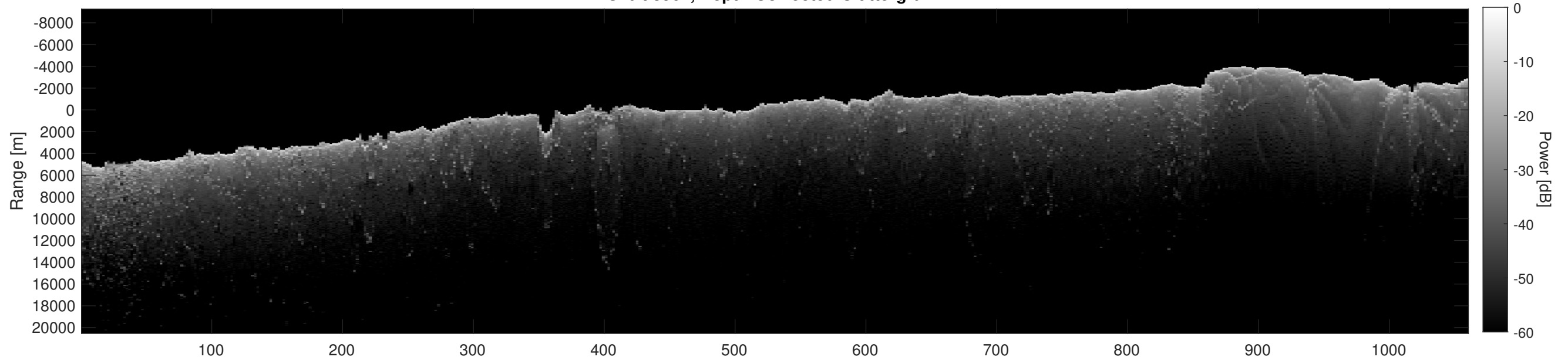
Orbit 8967, Depth-Corrected Cluttergram
