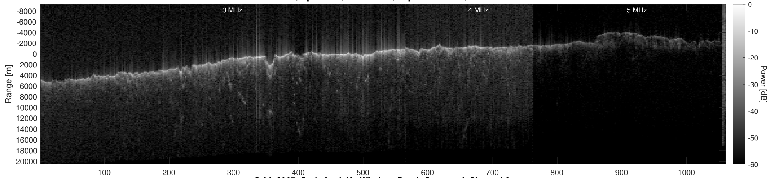
Orbit 8967, Optimized, No Window, Depth-Corrected, Channel 2
