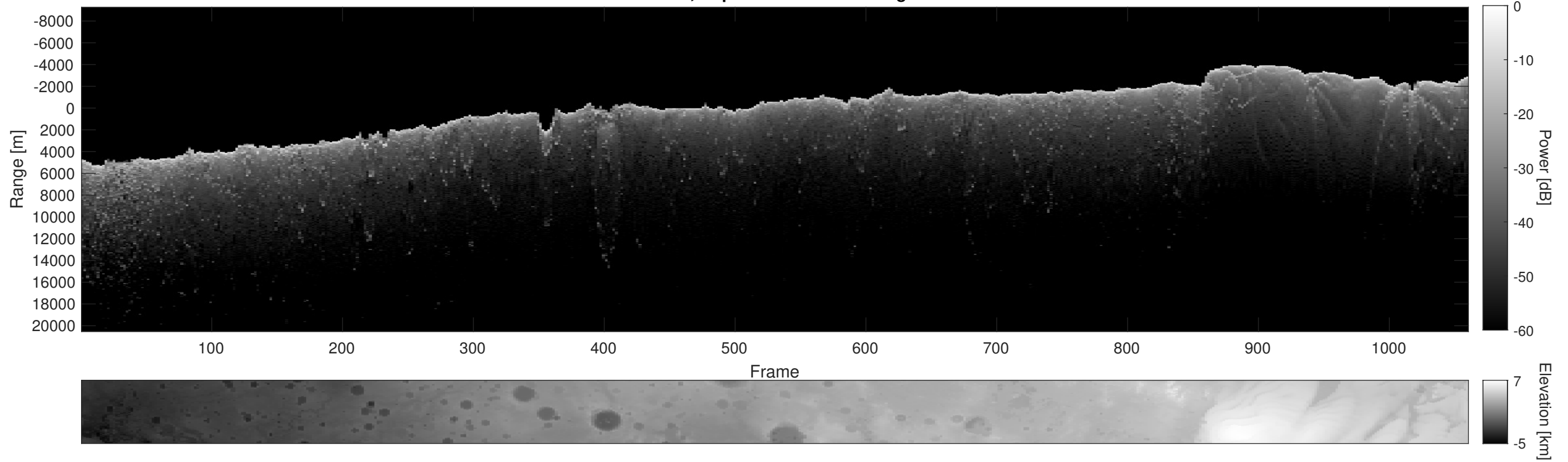
Orbit 8967, Depth-Corrected Cluttergram
