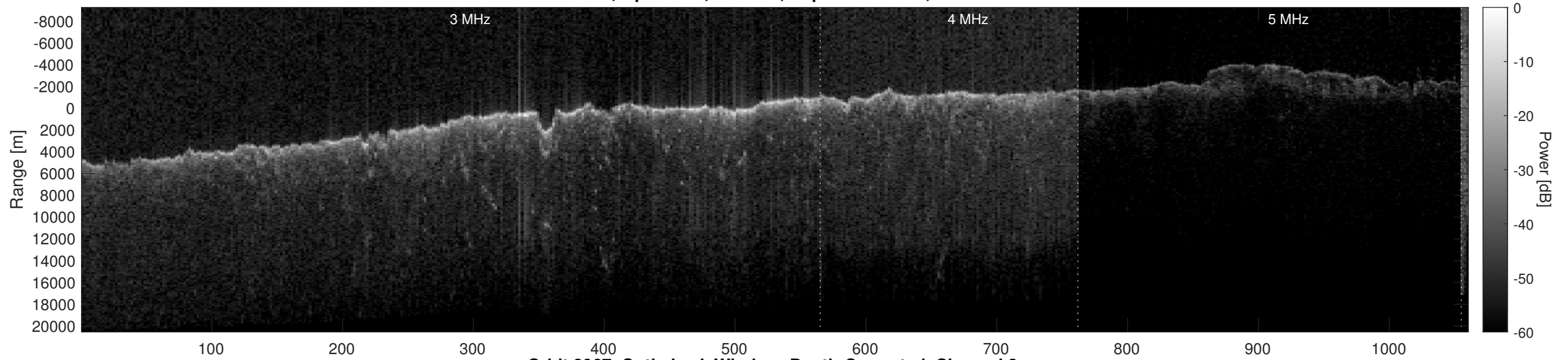
Orbit 8967, Optimized, Window, Depth-Corrected, Channel 2
