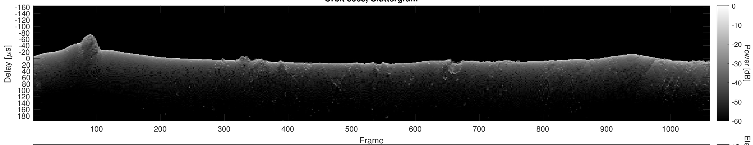
Orbit 8968, Cluttergram
