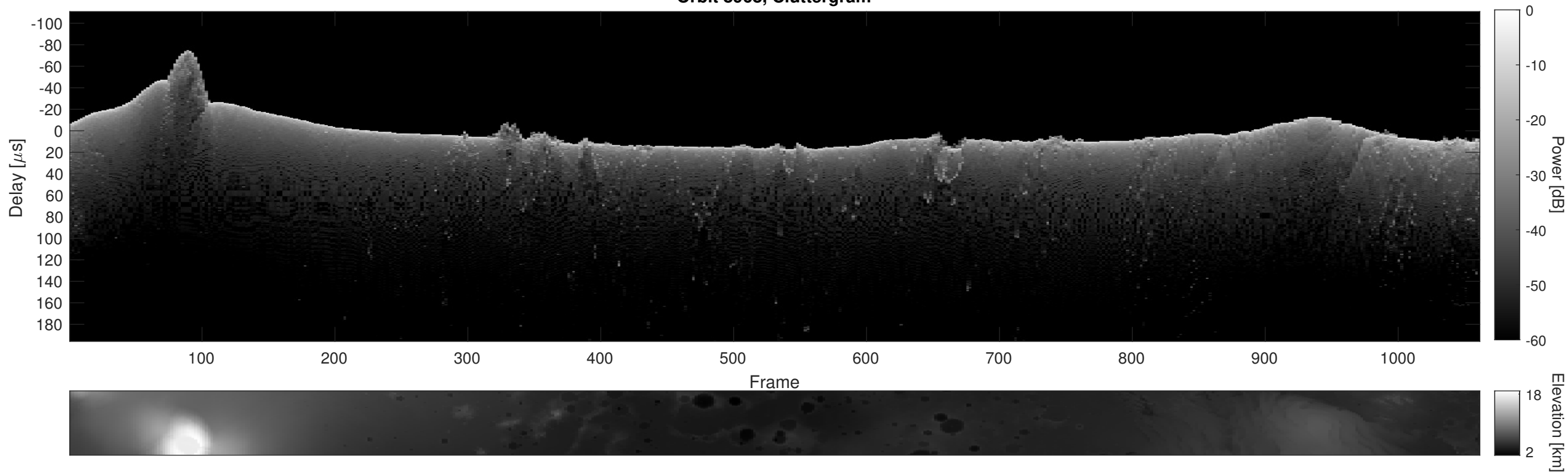
Orbit 8968, Cluttergram
