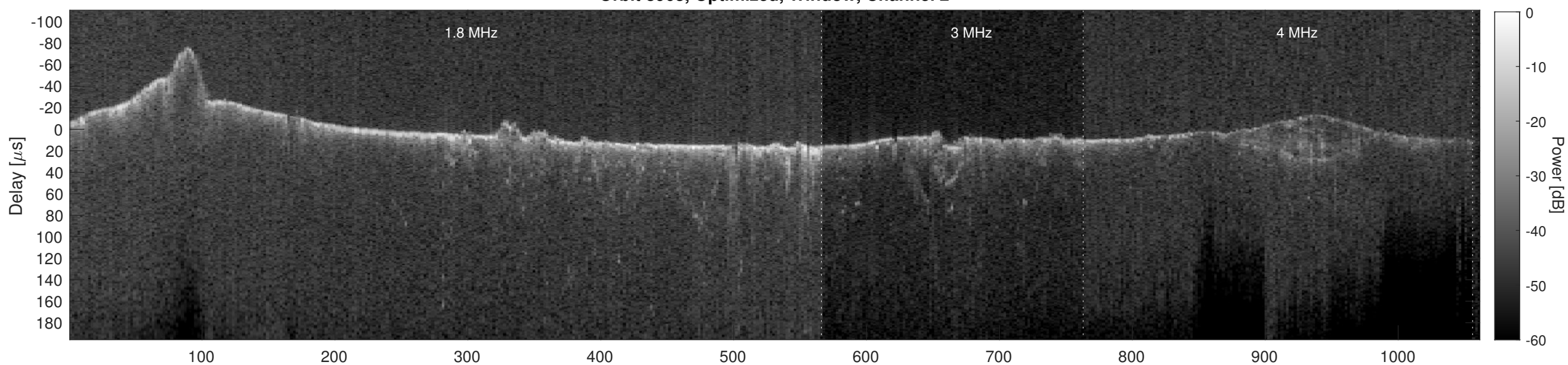
Orbit 8968, Cluttergram
