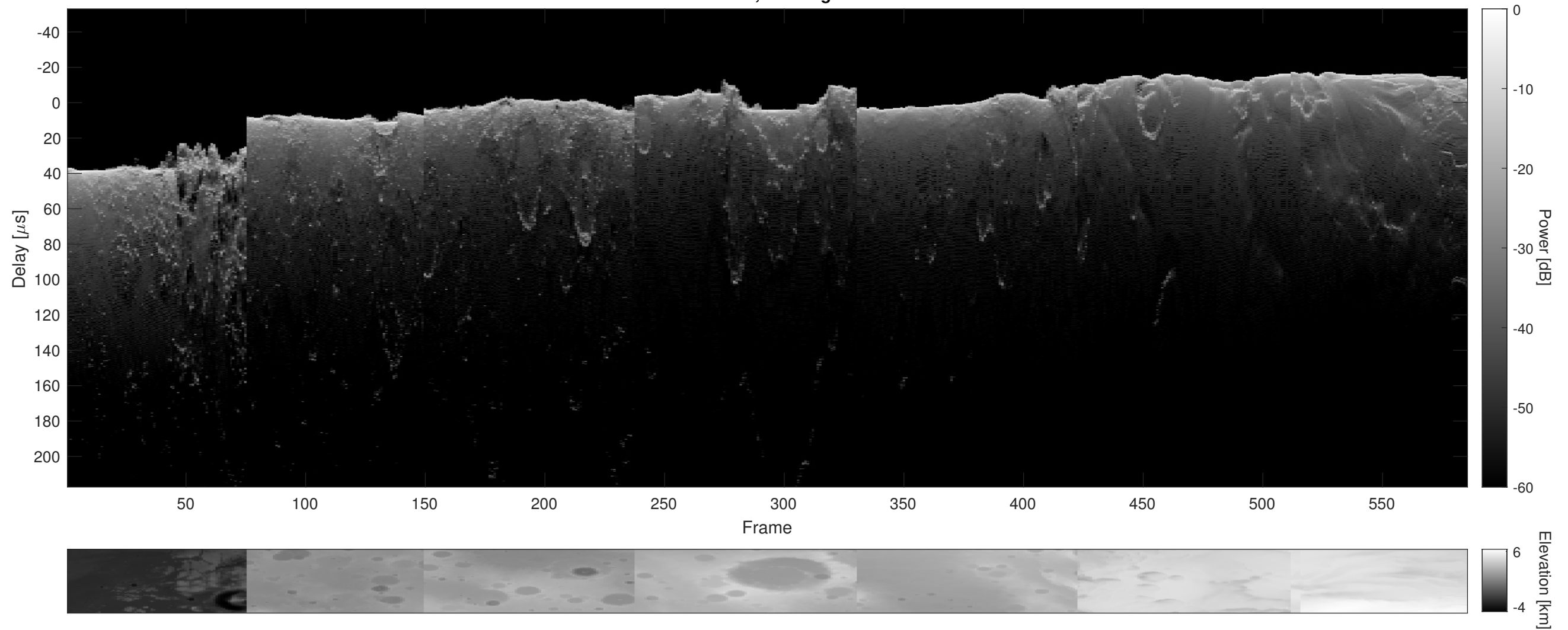
Orbit 8969, Cluttergram
