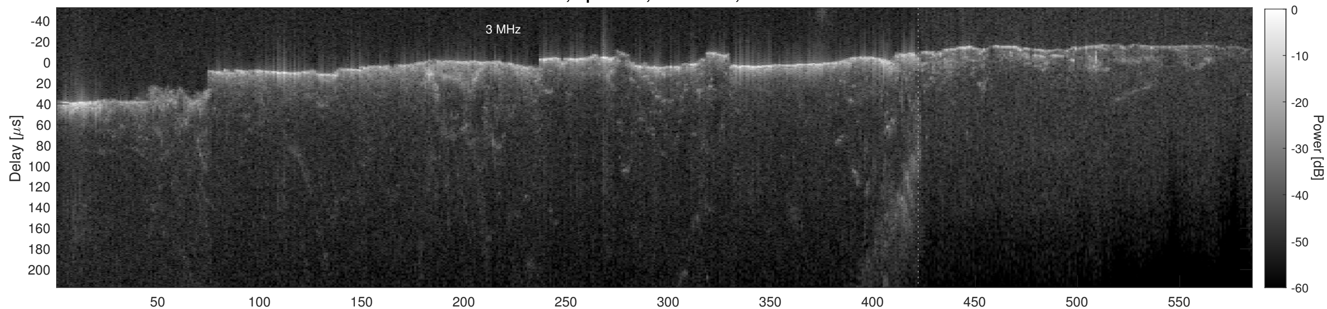
Orbit 8969, Cluttergram
