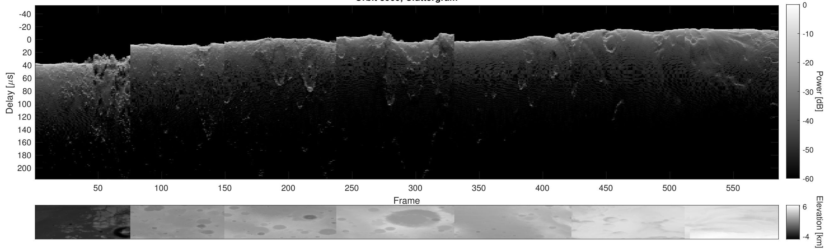
Orbit 8969, Cluttergram
