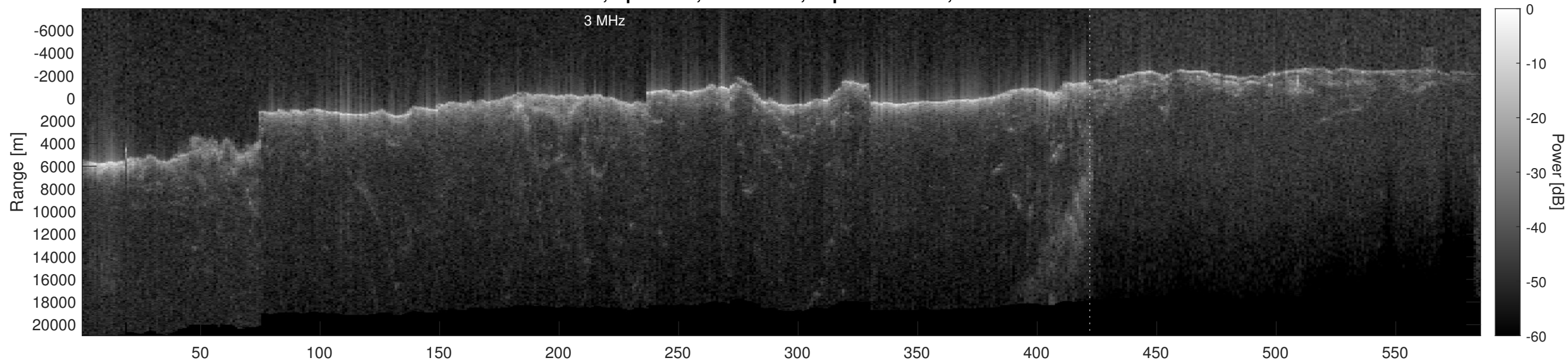
Orbit 8969, Optimized, No Window, Depth-Corrected, Channel 2
