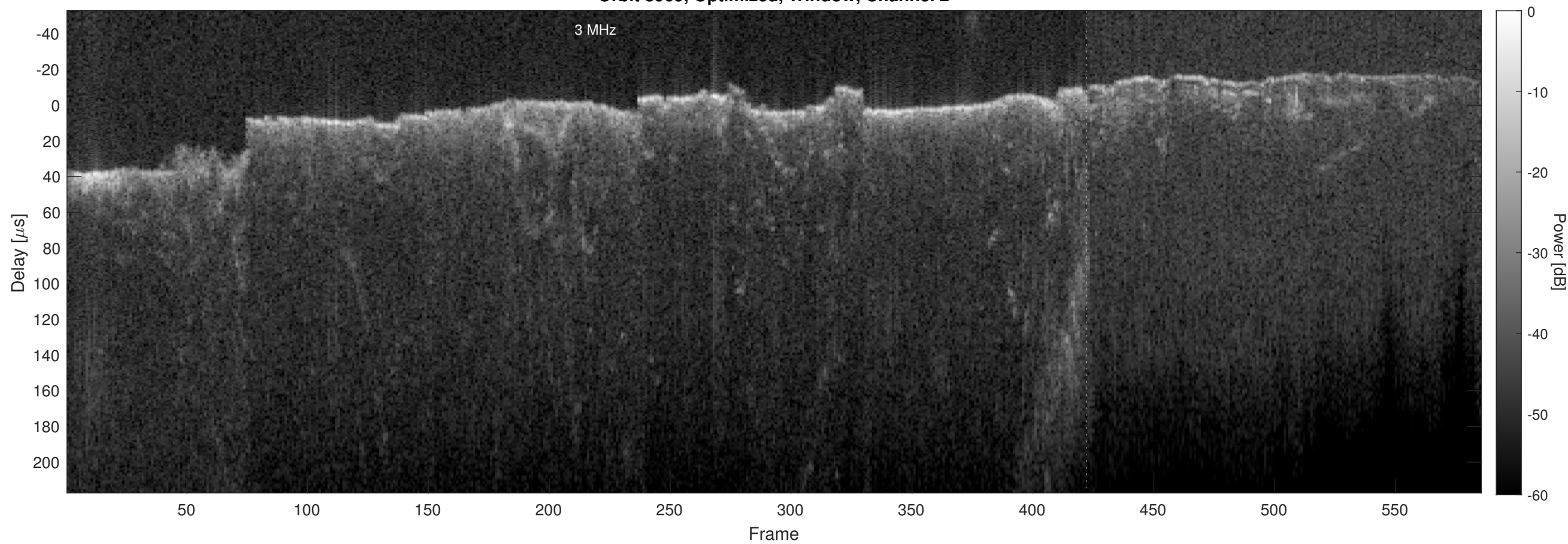
Orbit 8969, Optimized, Window, Channel 2
