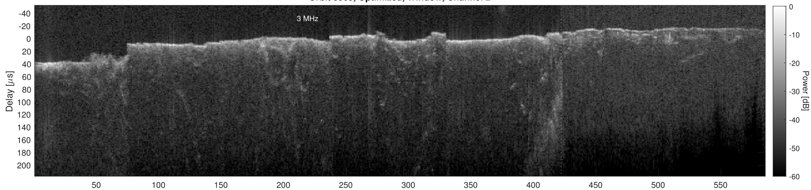
Orbit 8969, Cluttergram
