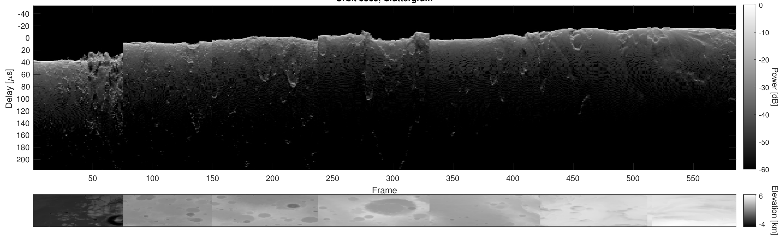
Orbit 8969, Cluttergram
