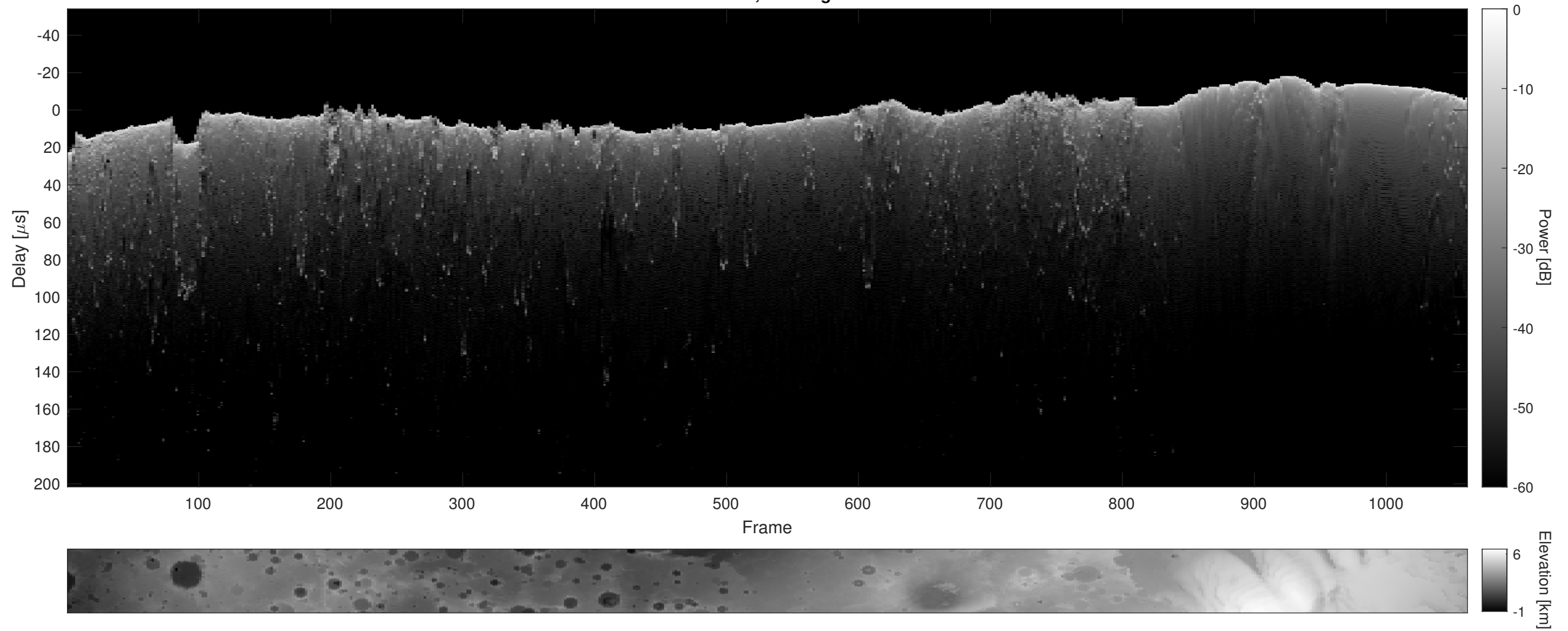
Orbit 8970, Cluttergram
