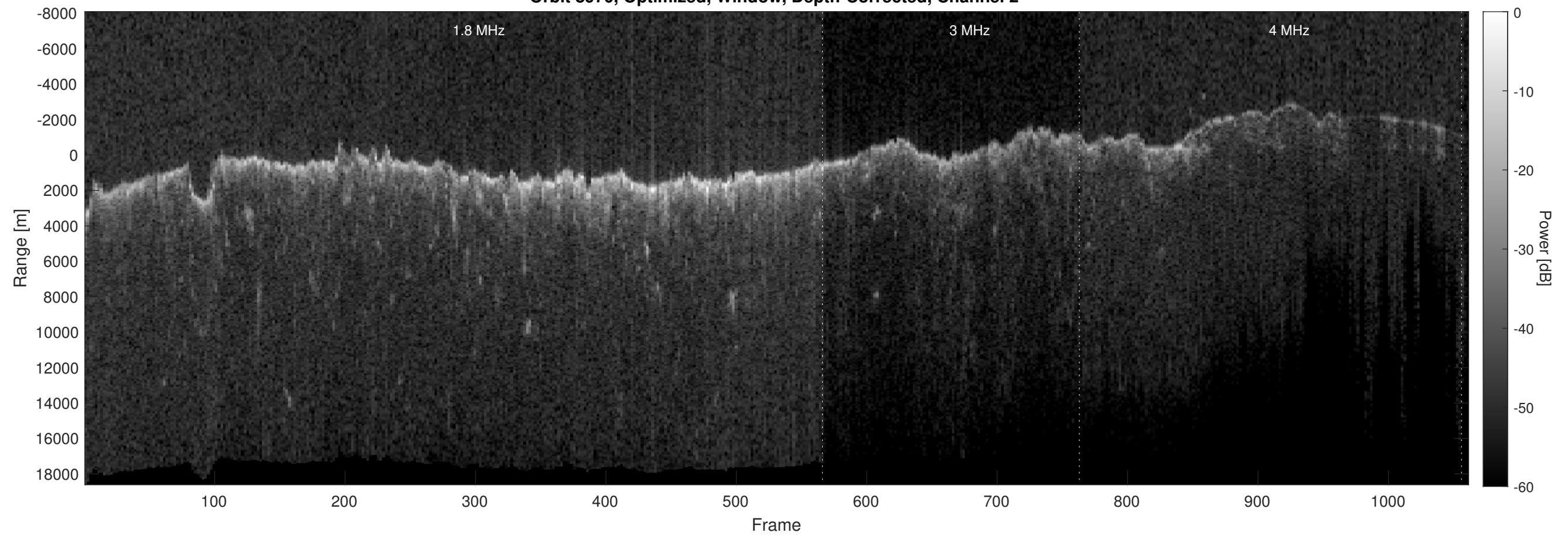
Orbit 8970, Optimized, Window, Depth-Corrected, Channel 2
