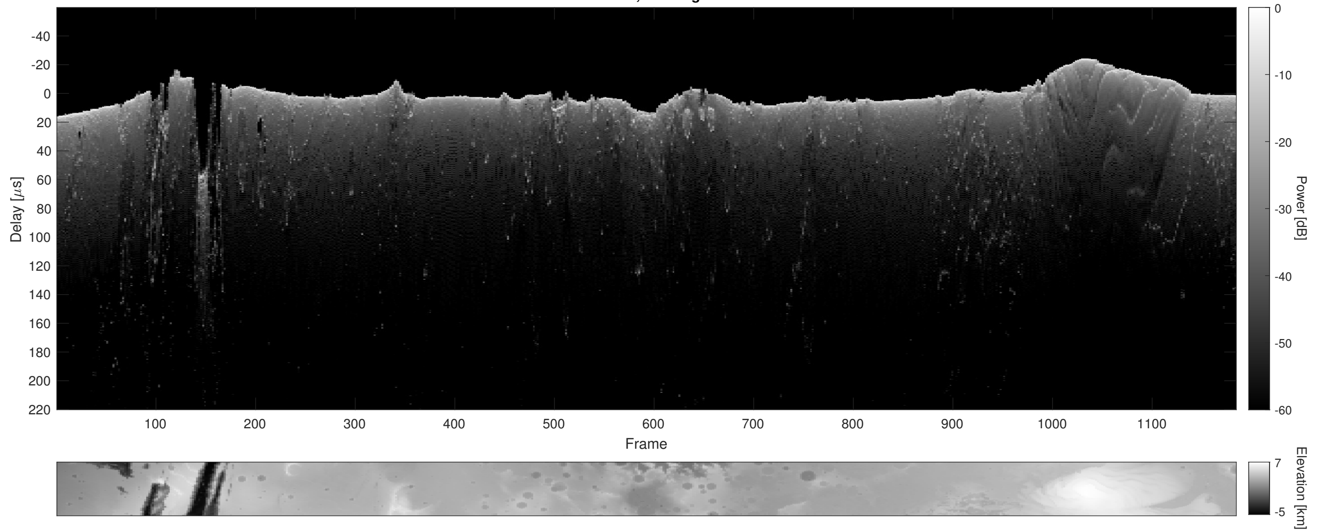
Orbit 8971, Cluttergram
