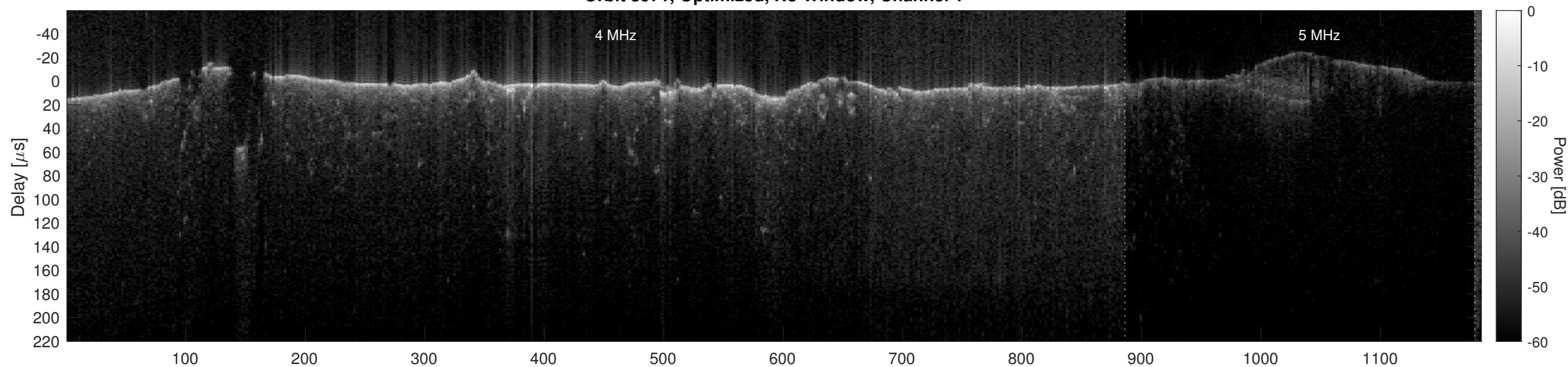
Orbit 8971, Optimized, No Window, Channel 2
