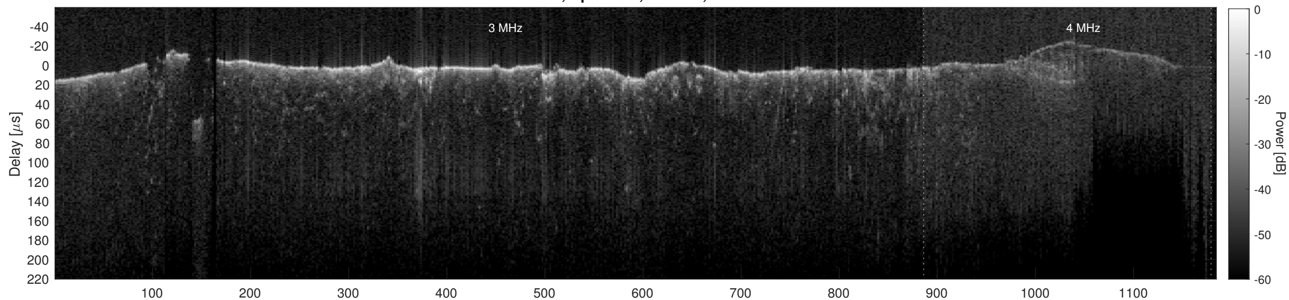
Orbit 8971, Cluttergram
