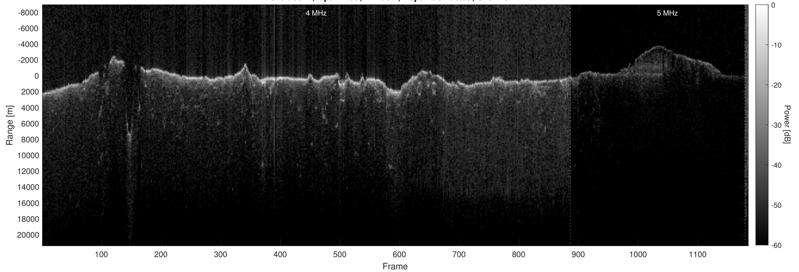
Orbit 8971, Optimized, Window, Depth-Corrected, Channel 2
