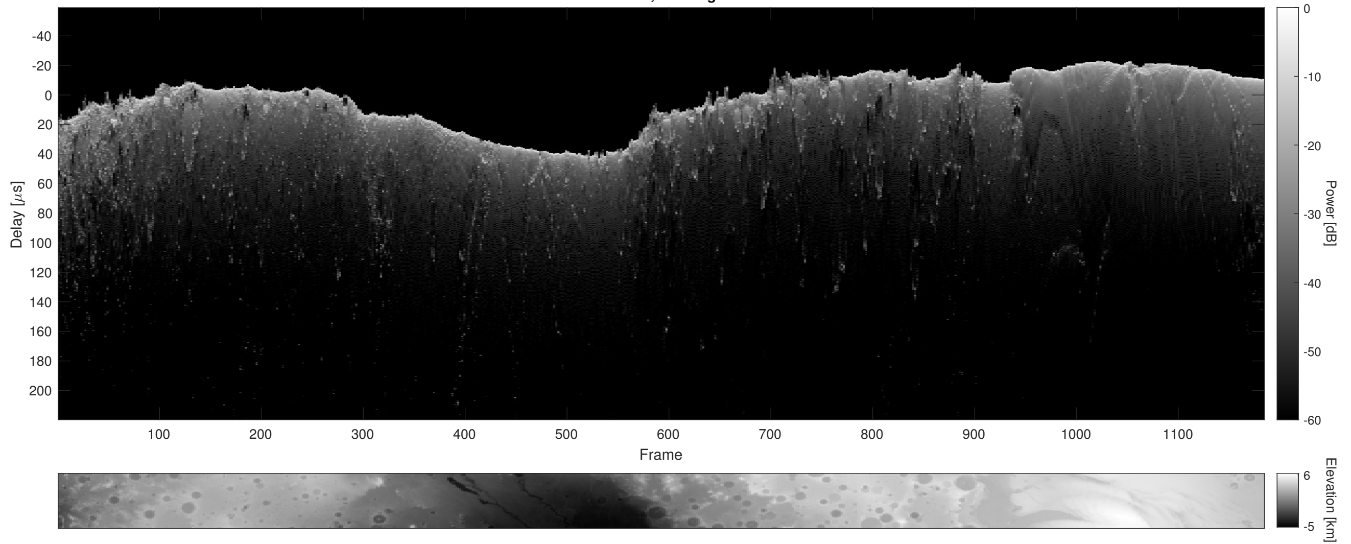
Orbit 8973, Cluttergram
