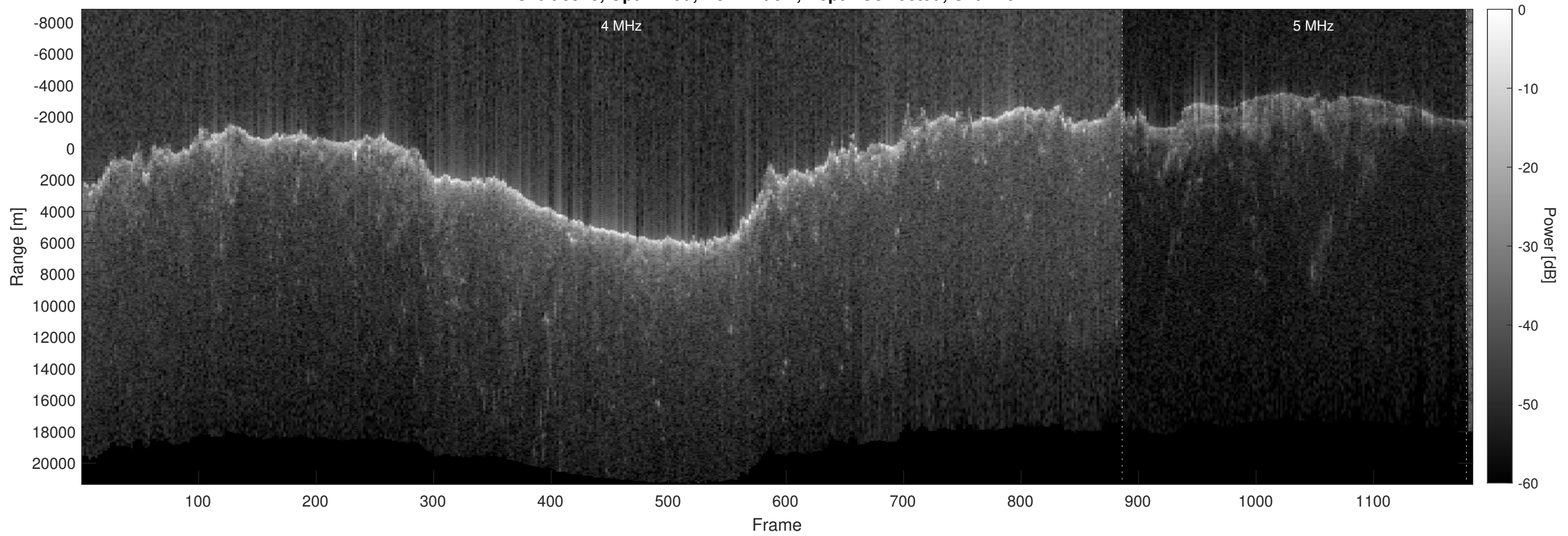
Orbit 8973, Optimized, No Window, Depth-Corrected, Channel 2
