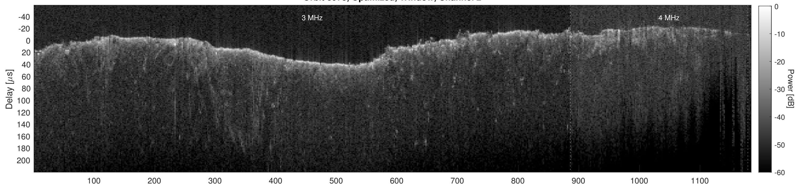
Orbit 8973, Cluttergram
