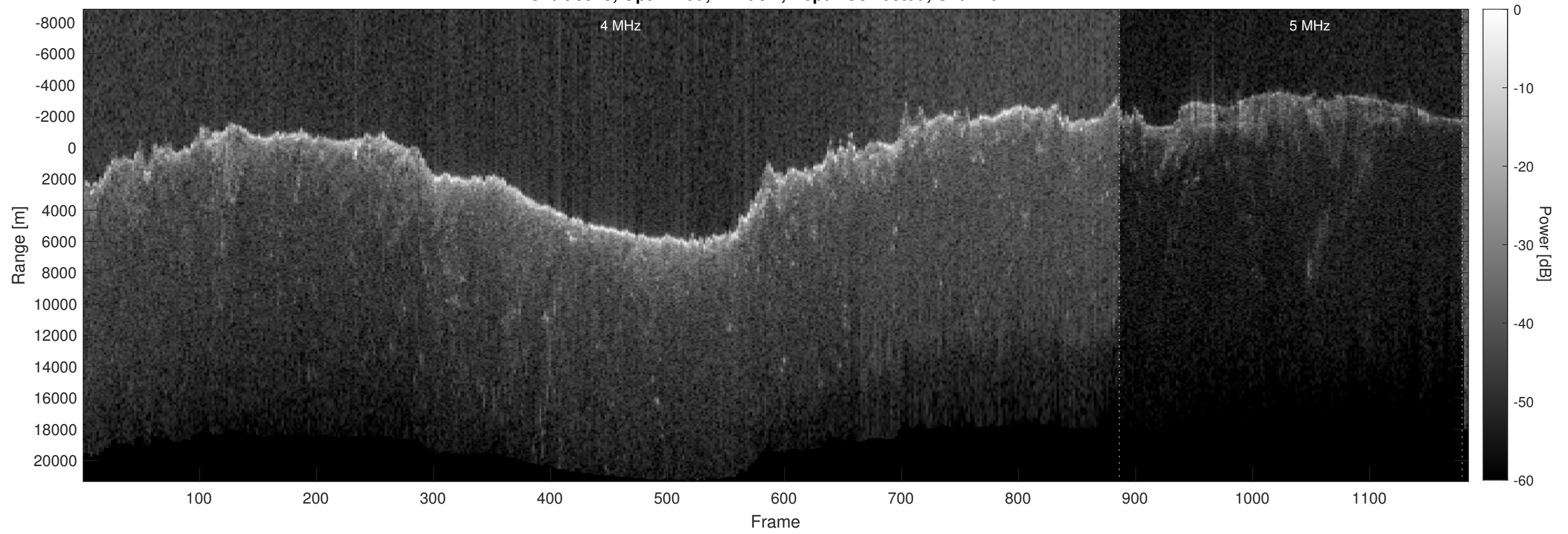
Orbit 8973, Optimized, Window, Depth-Corrected, Channel 2
