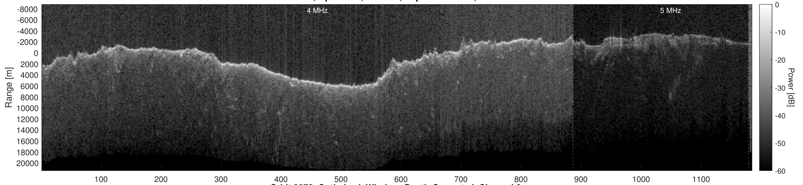
Orbit 8973, Optimized, Window, Depth-Corrected, Channel 2
