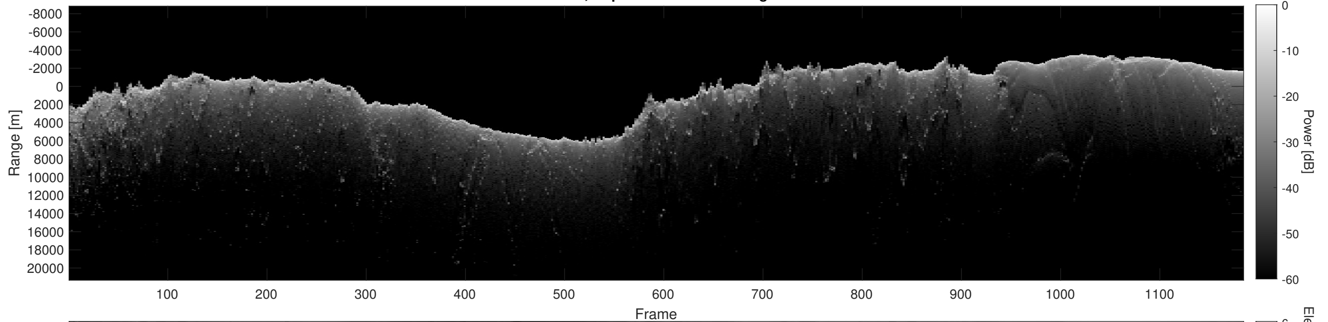
Orbit 8973, Depth-Corrected Cluttergram
