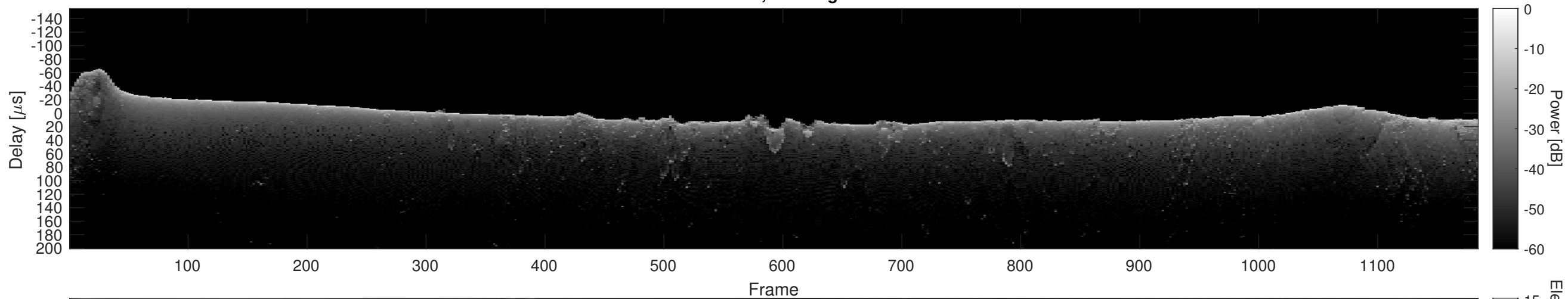
Orbit 8975, Cluttergram
