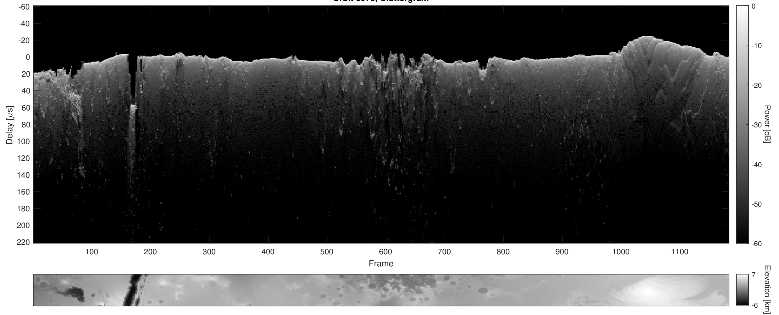
Orbit 8978, Cluttergram
