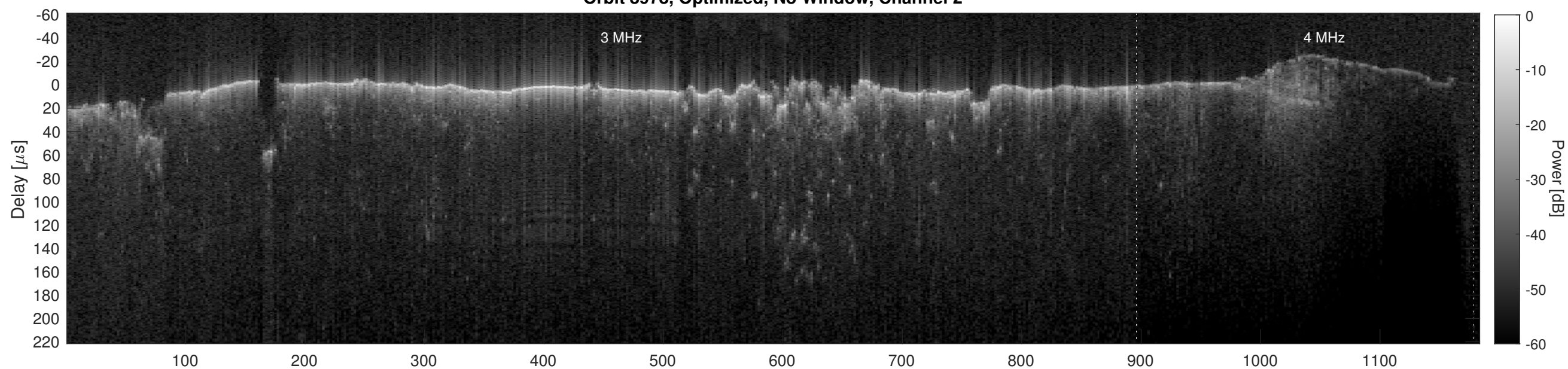
Orbit 8978, Cluttergram
