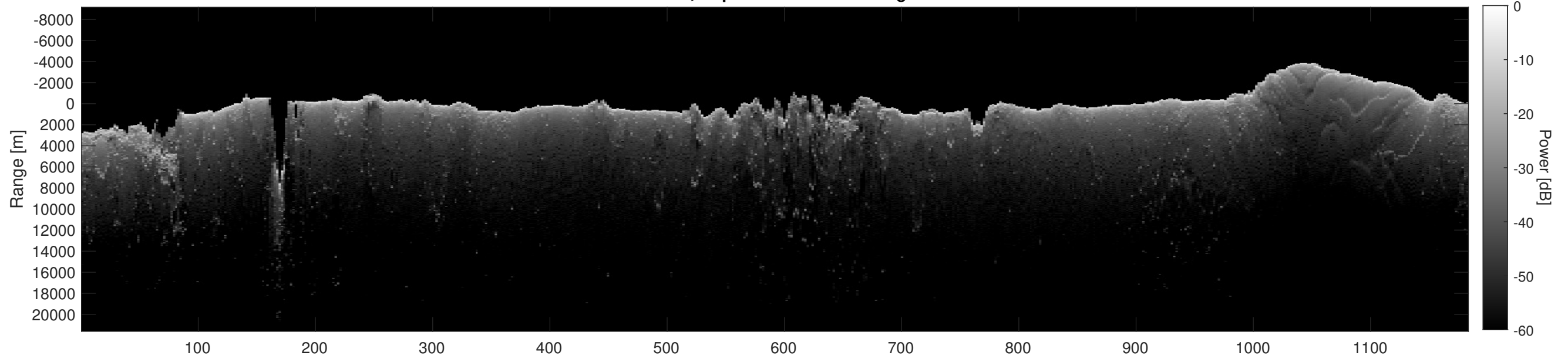
Orbit 8978, Depth-Corrected Cluttergram
