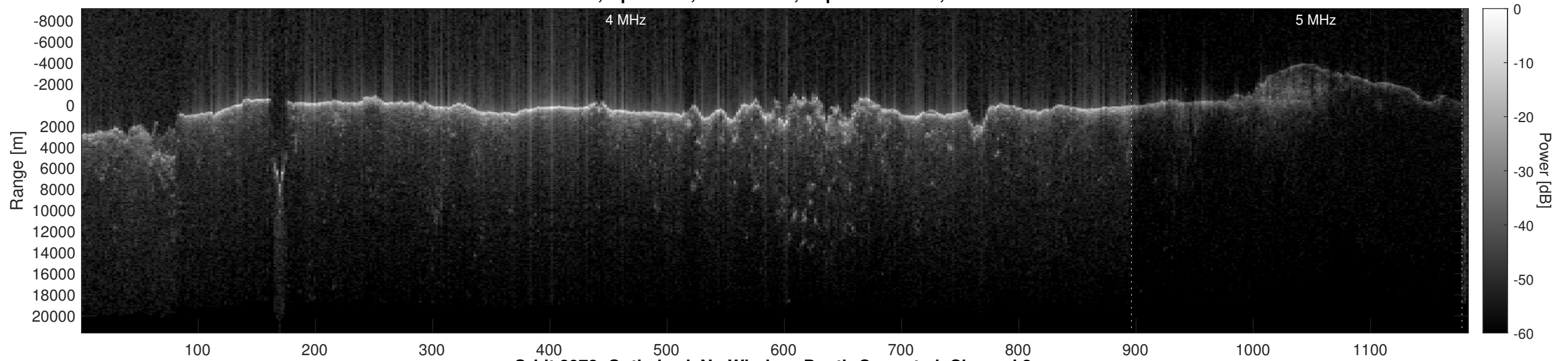
Orbit 8978, Optimized, No Window, Depth-Corrected, Channel 2
