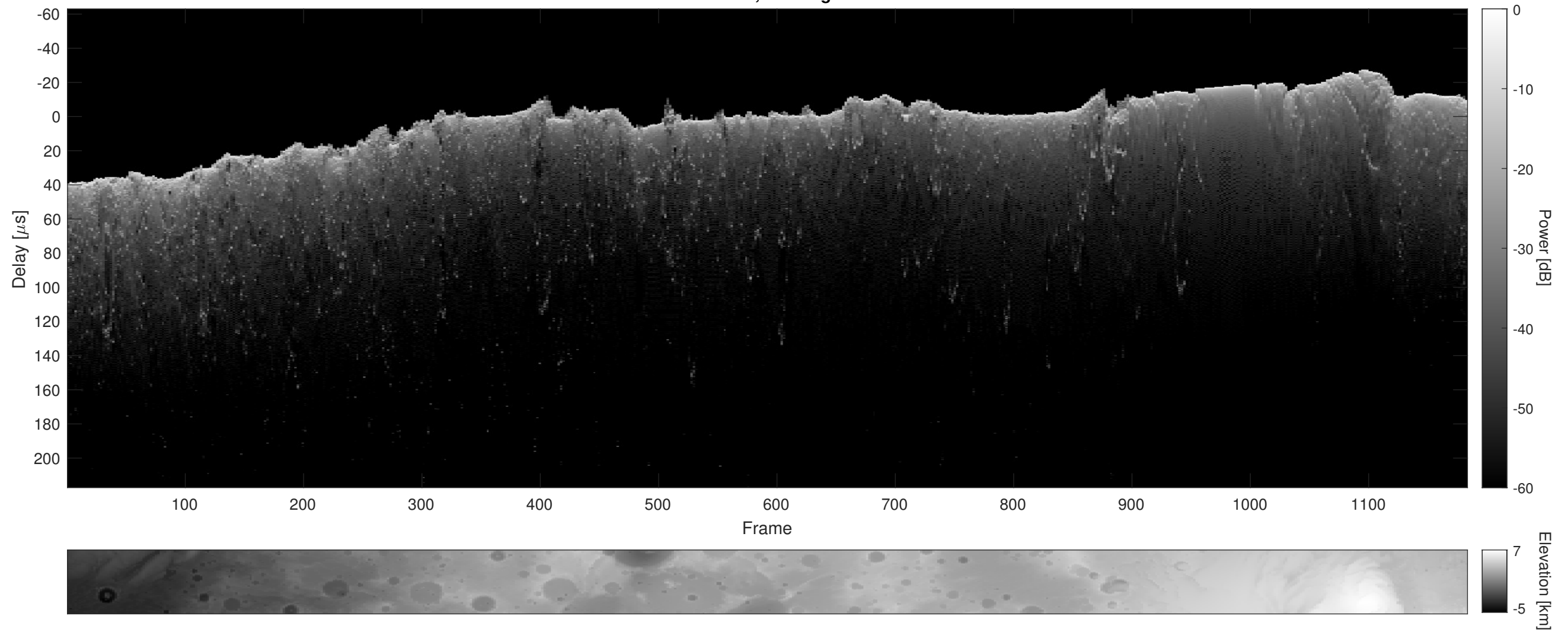
Orbit 8979, Cluttergram
