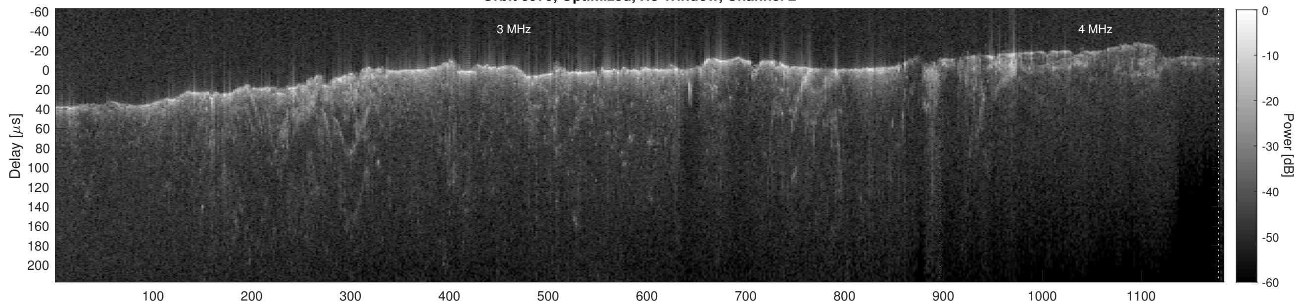
Orbit 8979, Cluttergram
